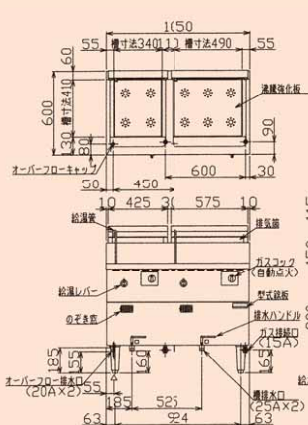
MRF-106C (2 槽式)
